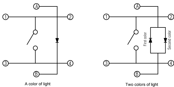
CIRCUIT DIAGRAM
